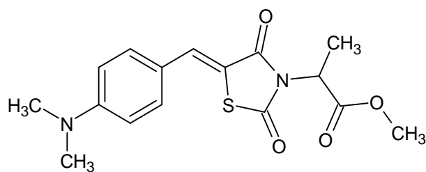
O=C1C(=C/c2ccc(cc2)N(C)C)/SC(=O)N1C(C)C(=O)OC Compound 15
