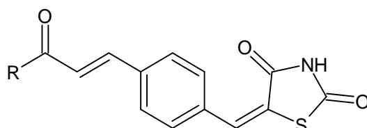
O=C1NC(=O)S\C1=C\c1ccc(/C=C/C([*])=O)cc1 Compound 4
