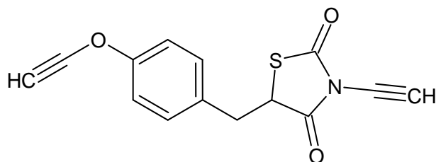
C#COc1ccc(CC2SC(=O)N(C#C)C2=O)cc1 Compound 12
