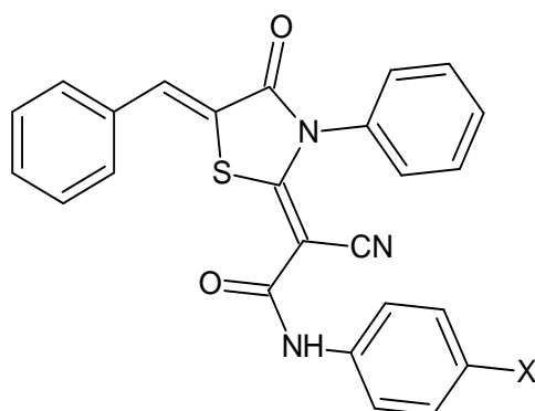
O=C(Nc1ccc([X])cc1)C(\C#N)=C1/S/C(=C/c2ccccc2)C(=O)N1c1ccccc1 Compound 3
