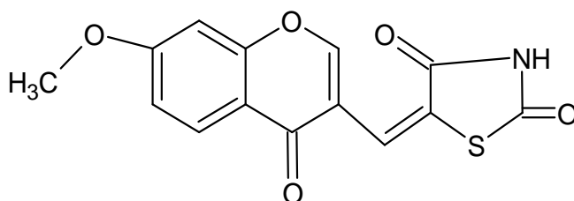
O=C1NC(=O)S\C1=C\C1=COc2cc(OC)ccc2C1=O Compound 13
