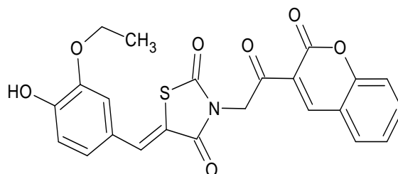
O=C(CN1C(=O)C(=C/c2ccc(O)c(OCC)c2)/SC1=O)C1=Cc2ccccc2OC1=O Compound 20
