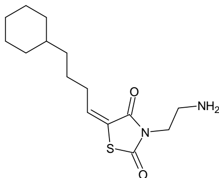
Compound 5
