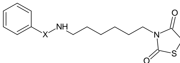
O=C1CSC(=O)N1CCCCCCN[X]c1ccccc1 Compound 10
