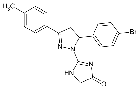
Brc1ccc(cc1)C1CC(=NN1C(=O)N)C1 Compound 9
