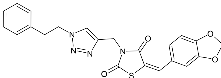
O=C1S/C(=C/c2ccc3OCOc3c2)C(=O)N1Cc1nnn(CCc2ccccc2)c1 Compound 11
