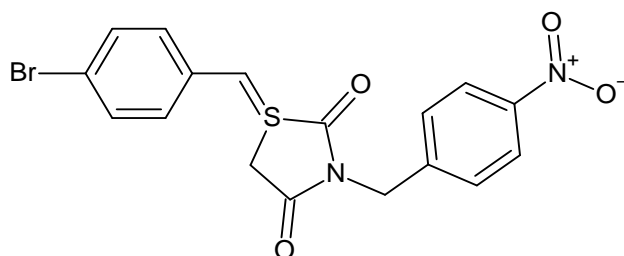
Compound 6
