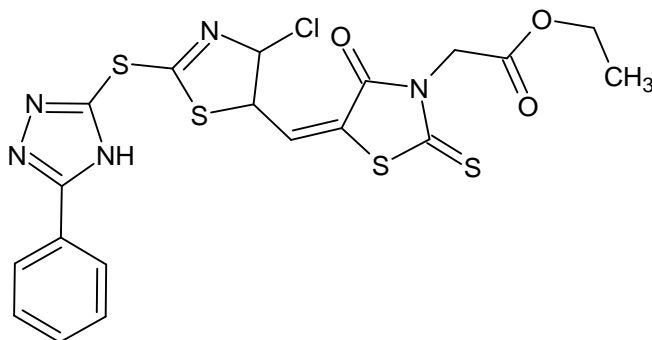
O=C(OCC)CN1C(=S)S/C(=C/C2SC(=NC2Cl)Sc2nnc([NH]2)c2ccccc2)C1=O Compound 14
