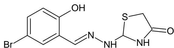
Brc1cc(/C=N/NC2NC(=O)CS2)c(O)cc1 Compound 8
