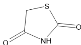
1,3-thiazolidine-2,4-dione
