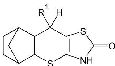
O=C1SC=2C([*])C3C4CC(CC4)C3SC=2N1 Compound 1
