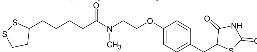
O=C1NC(=O)SC1Cc1ccc(cc1)OCCN(C)C(=O)CCCCC1CCSS1 Compound 2
