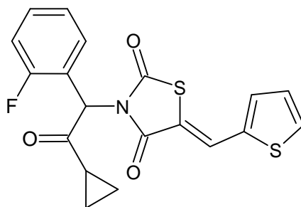
O=C(C(N1C(=O)C(=C/c2cccs2)/SC1=O)c1ccccc1F)C1CC1 Compound 18
