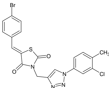
O=C1S\C(=C/c2ccc(Br)cc2)C(=O)N1Cc1nnn(c1)c1ccc(C)c(Cl)c1 Compound 17
