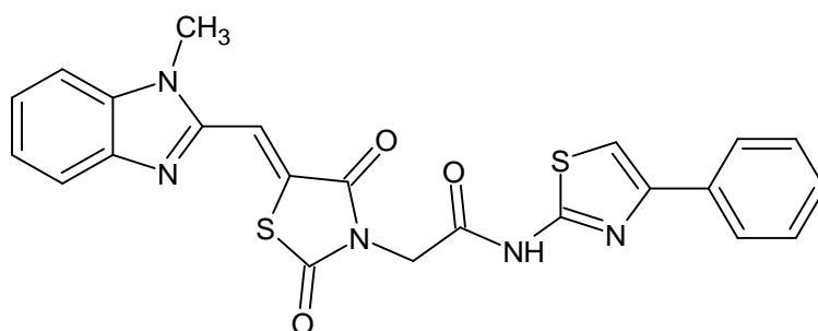
Compound 7
