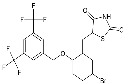
FC(F)(F)c1cc(cc(c1)C(F)(F)F)COC1CCC(Br)CC1CC1SC(=O)NC1=O Compound 19
