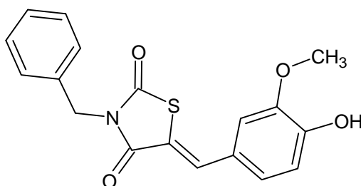
O=C1S\C(=C/c2ccc(O)c(OC)c2)C(=O)N1Cc1ccccc1 Compound 16
