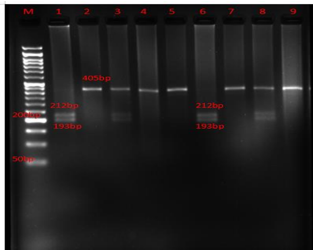
Fig 2: PCR RFLP analysis c.766C>G polymorphism in the of Fetuin A. Lane M: 50 bp marker; Lanes 1,6: GG alleles ;Lanes 2,4,5,7,9: CC alleles ; Lanes 3,8 :CG alleles
