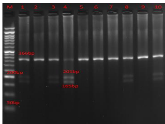
Fig 1: PCR RFLP analysis c.742C>T polymorphism in the of Fetuin A.Lane M: 50 bp marker: Lanes 1,3,8,10: CT alleles ;Lanes 2,5,6,7,9: CC alleles ; Lanes 4:TT alleles
